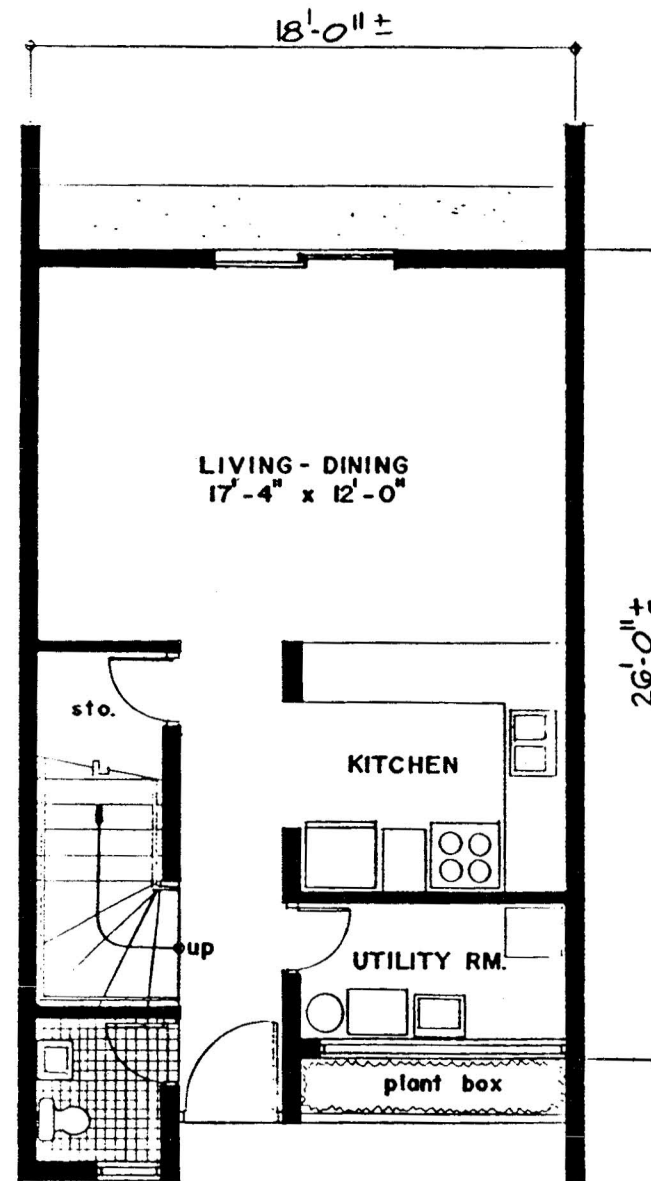
GROUND FLOOR
